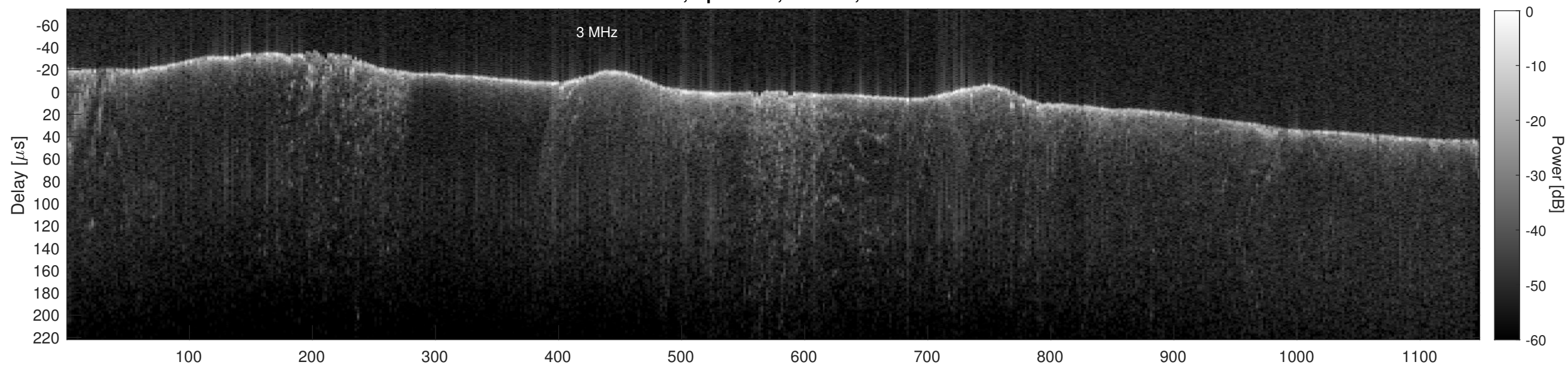
Orbit 3937, Cluttergram
