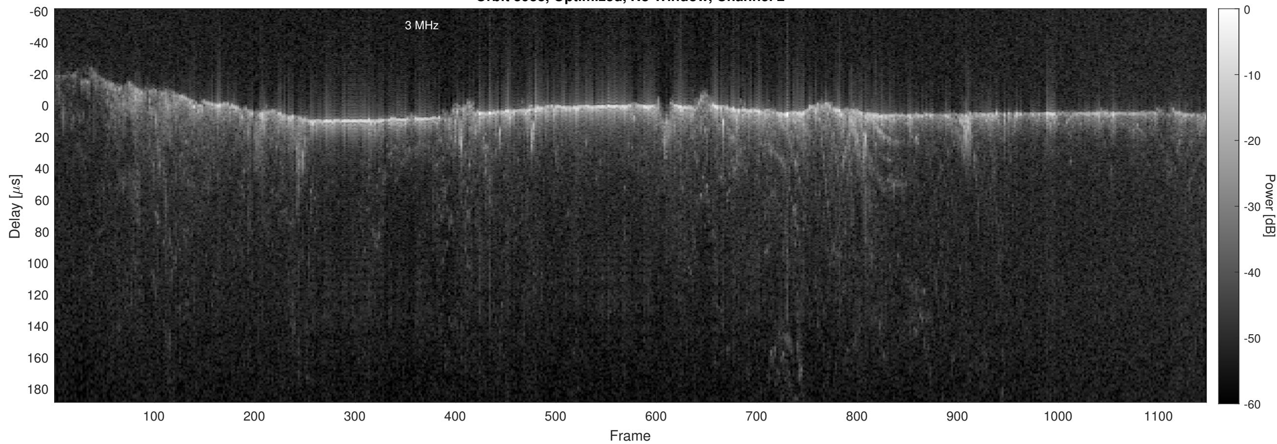
Orbit 3938, Optimized, No Window, Channel 2
