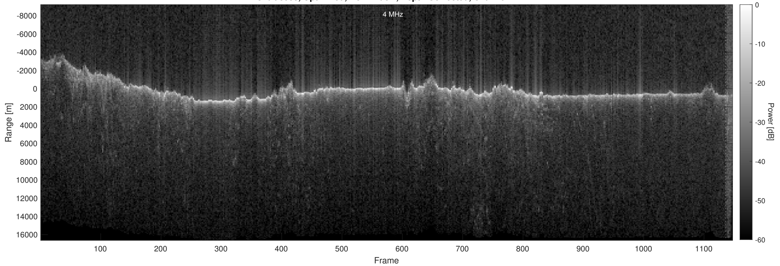
Orbit 3938, Optimized, No Window, Depth-Corrected, Channel 2
