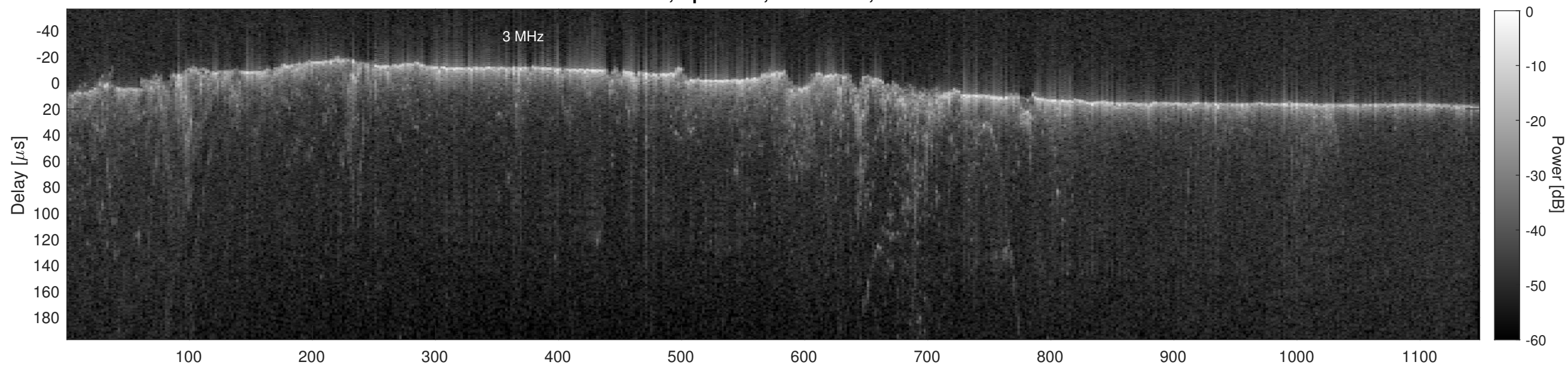
Orbit 3939, Cluttergram
