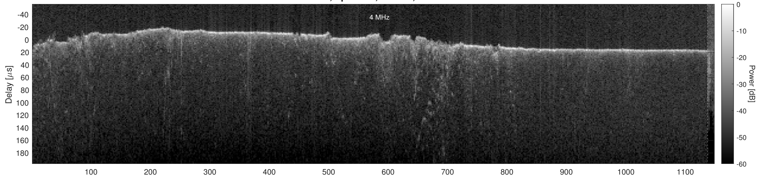
Orbit 3939, Optimized, Window, Channel 2
