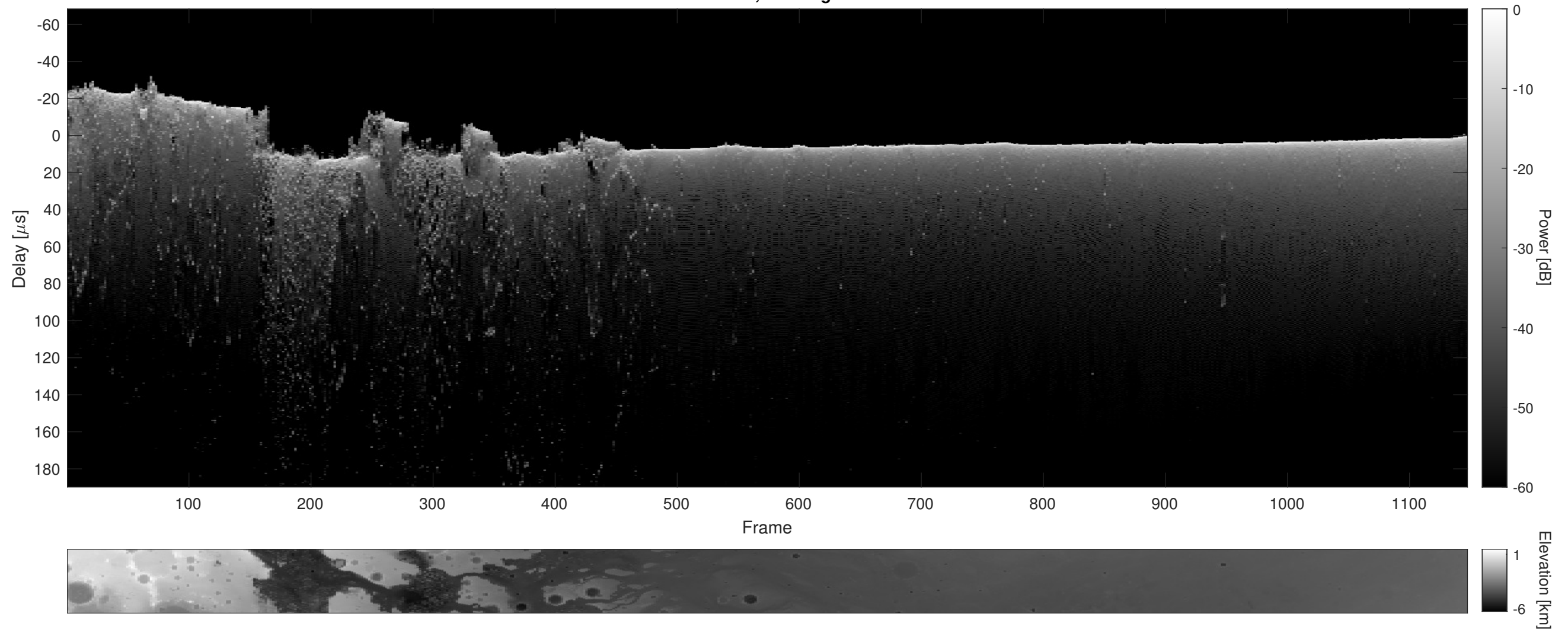
Orbit 3940, Cluttergram
