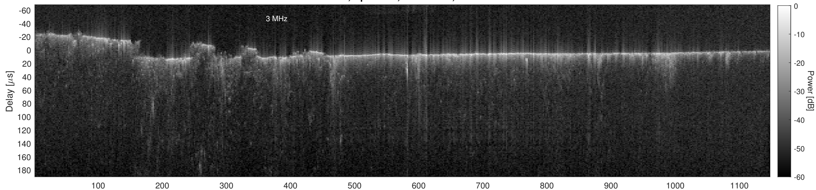
Orbit 3940, Cluttergram
