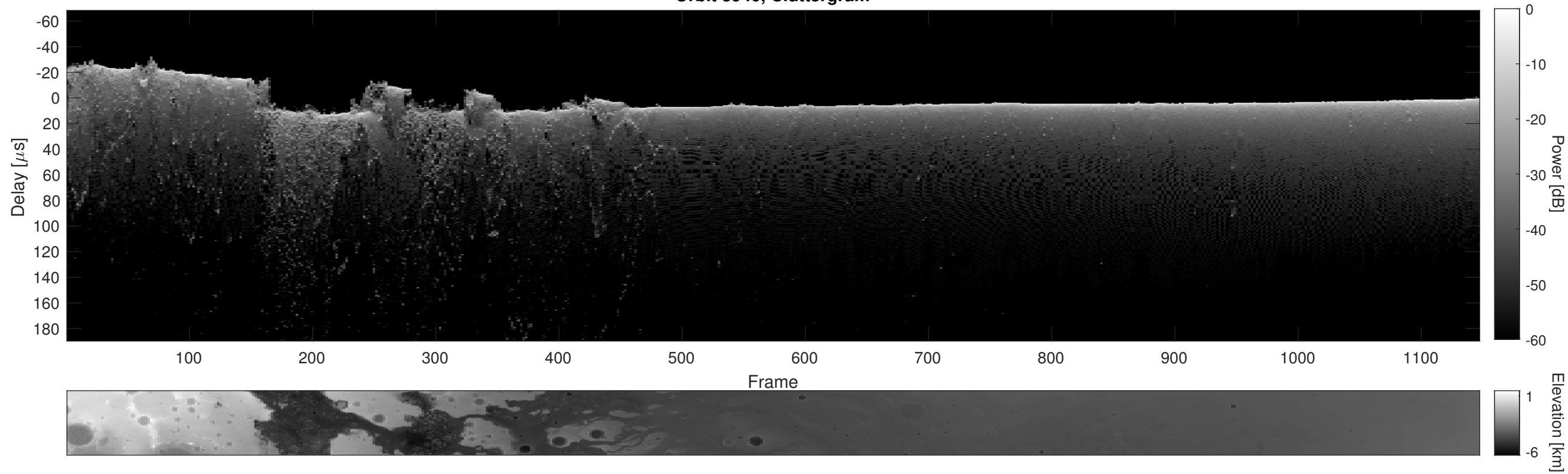
Orbit 3940, Cluttergram
