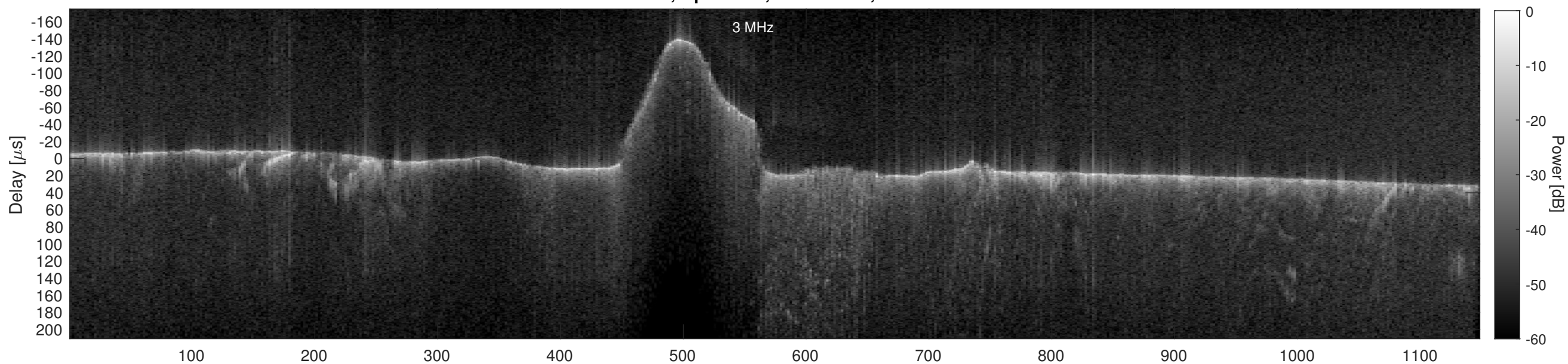
Orbit 3941, Cluttergram
