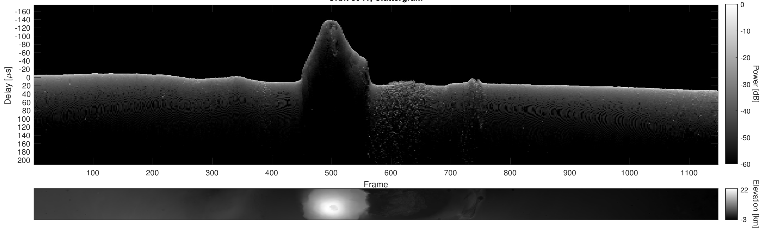
Orbit 3941, Cluttergram
