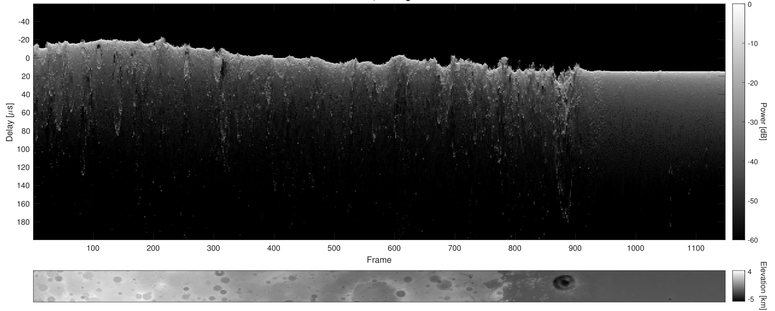
Orbit 3943, Cluttergram
