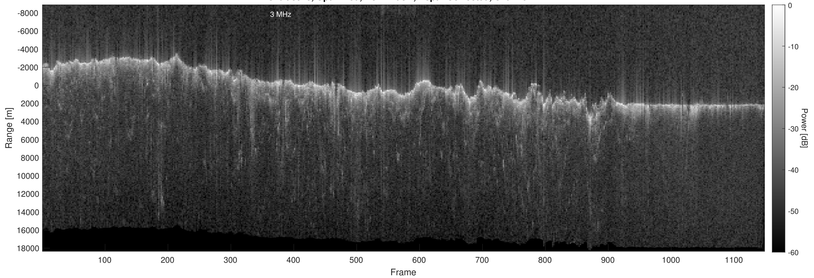
Orbit 3943, Optimized, No Window, Depth-Corrected, Channel 2
