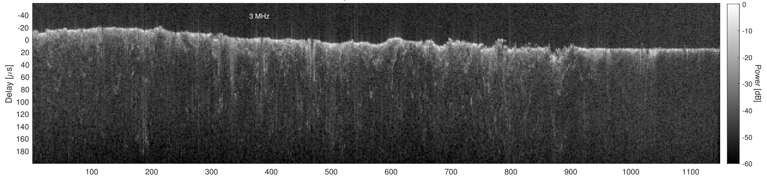
Orbit 3943, Cluttergram
