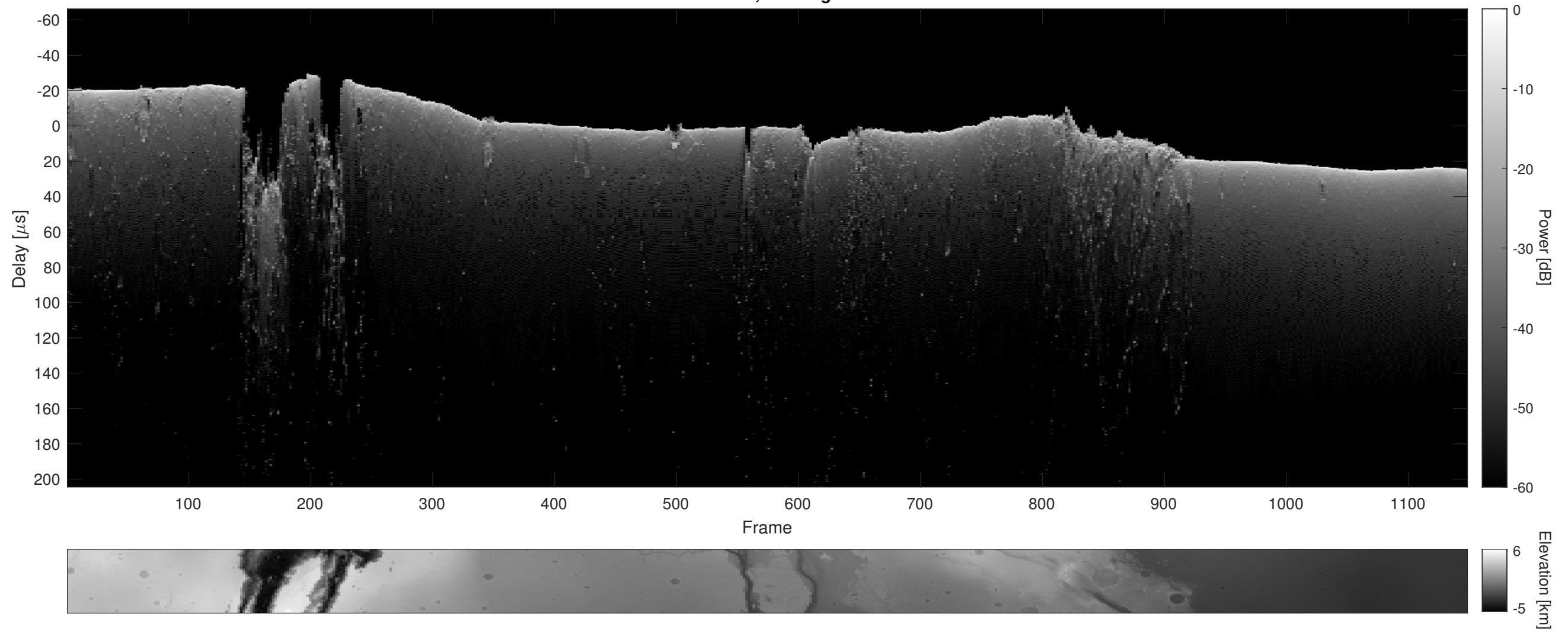
Orbit 3944, Cluttergram
