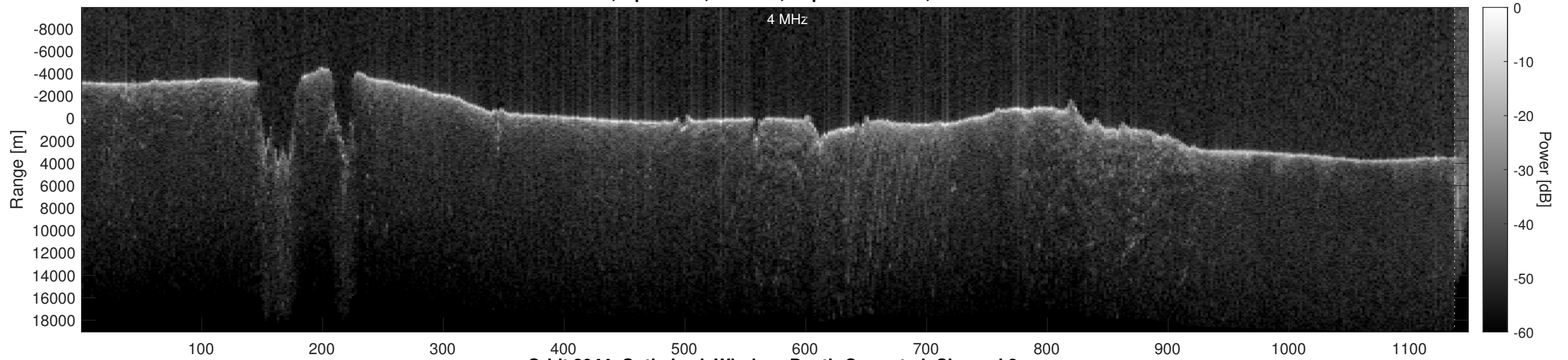
Orbit 3944, Optimized, Window, Depth-Corrected, Channel 2
