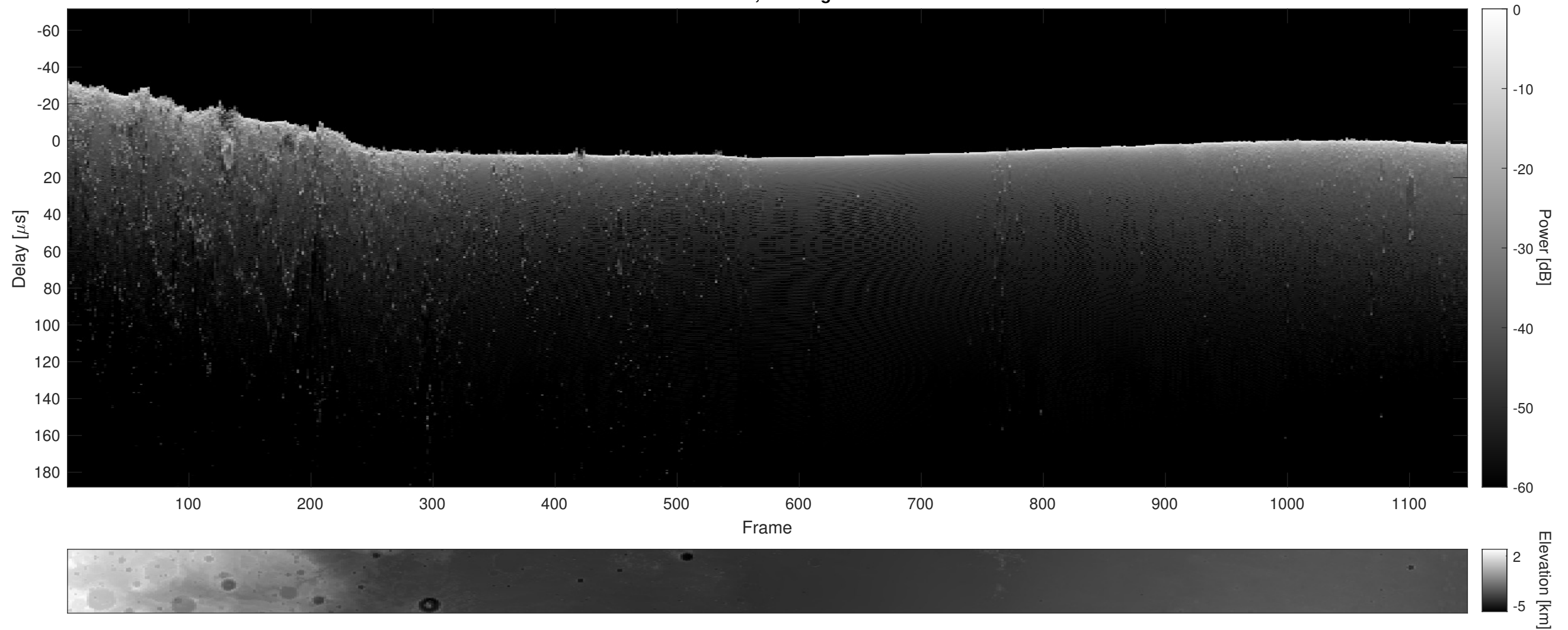
Orbit 3945, Cluttergram
