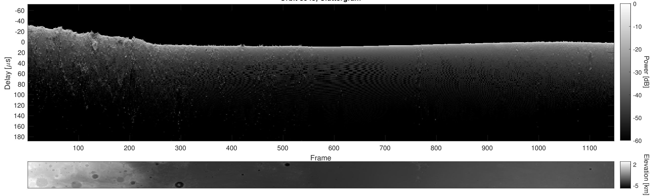
Orbit 3945, Cluttergram
