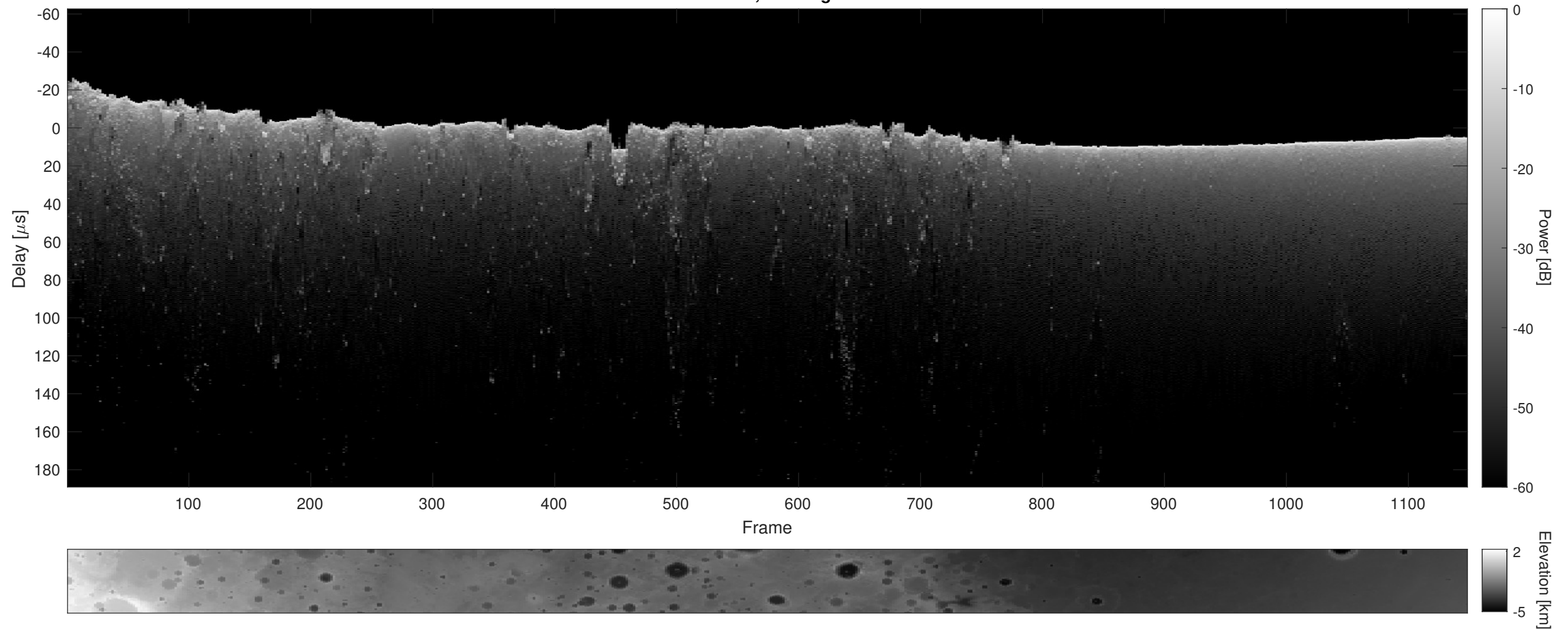
Orbit 3947, Cluttergram
