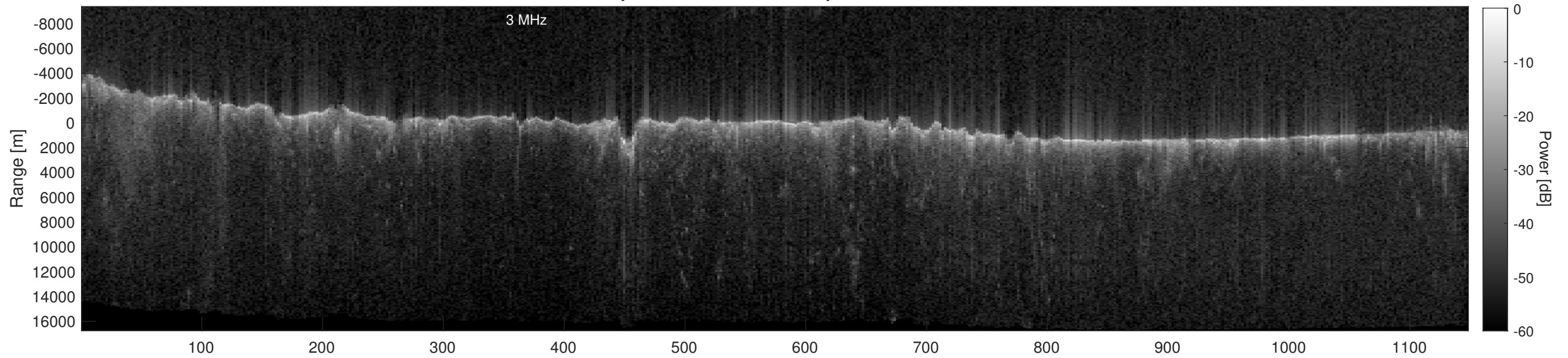
Orbit 3947, Depth-Corrected Cluttergram
