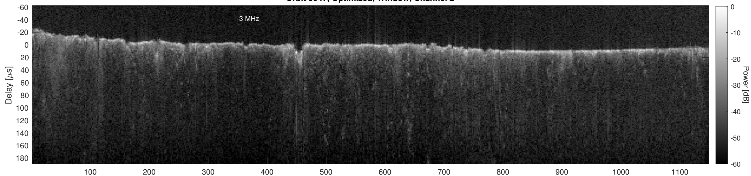
Orbit 3947, Cluttergram
