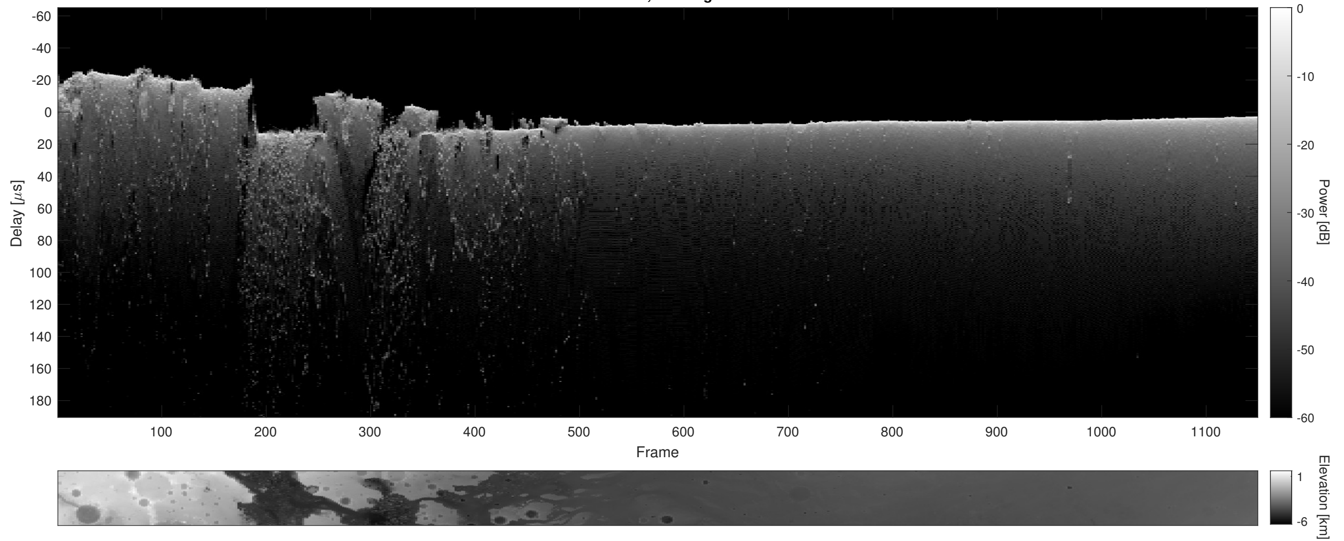
Orbit 3951, Cluttergram
