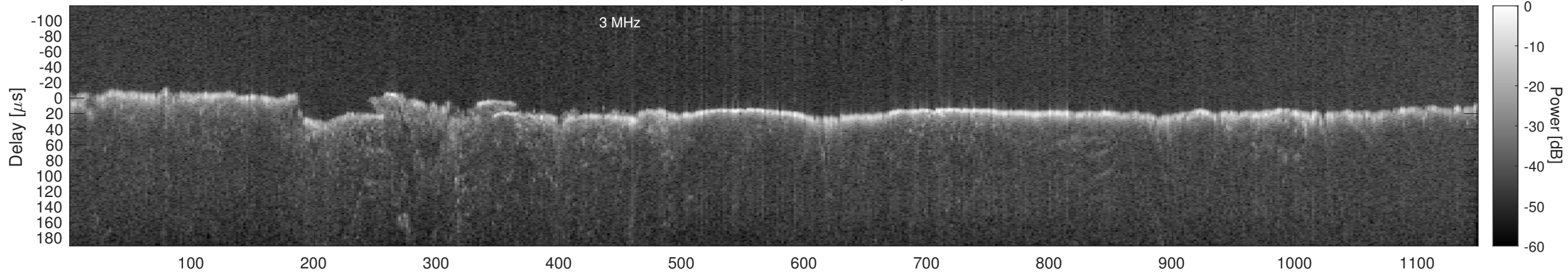
Orbit 3951, Window, Channel 2, Optimized
