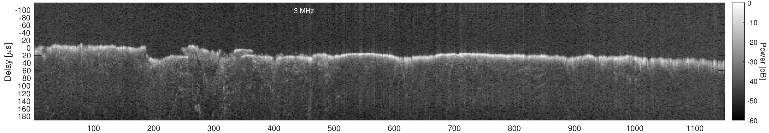
Orbit 3951, Window, Channel 2, Chapman
