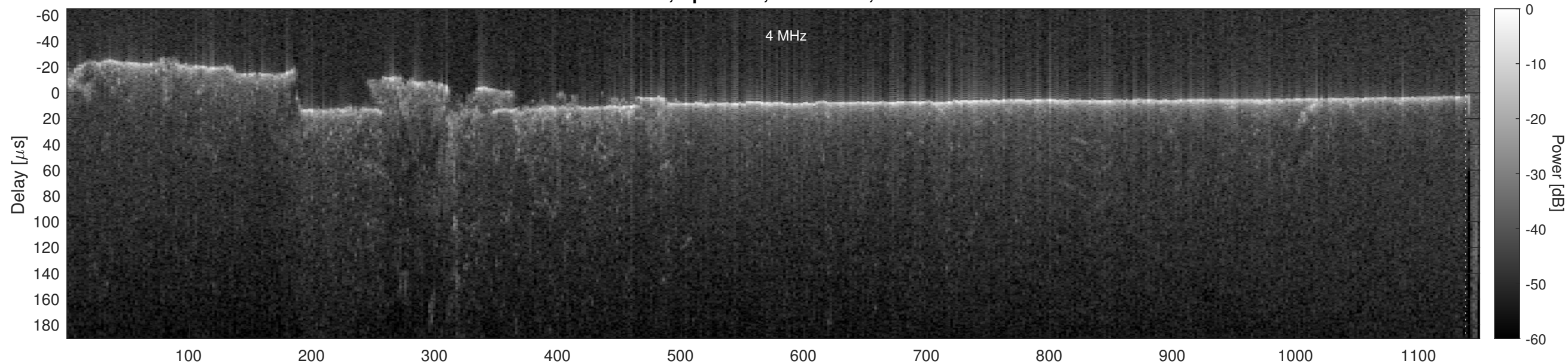
Orbit 3951, Optimized, No Window, Channel 2
