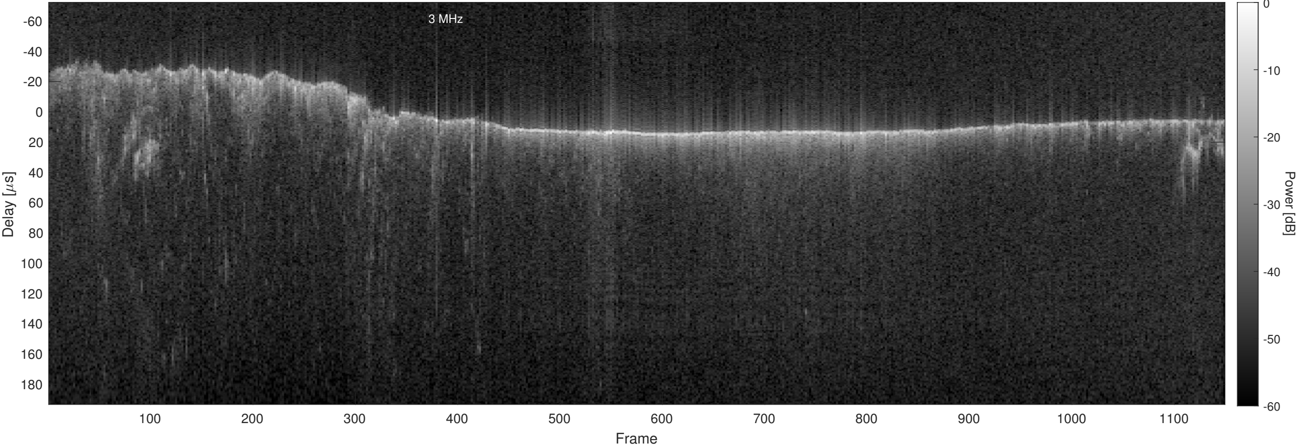
Orbit 3953, Optimized, No Window, Channel 2
