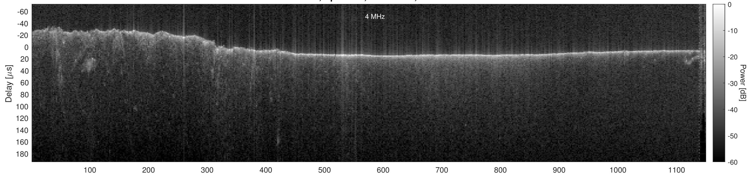
Orbit 3953, Optimized, No Window, Channel 2
