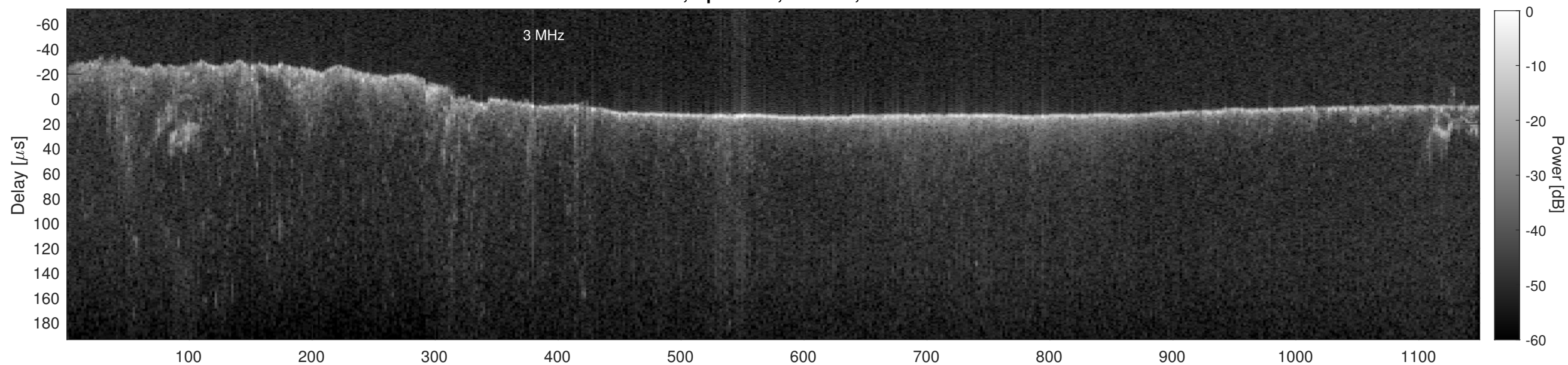
Orbit 3953, Cluttergram
