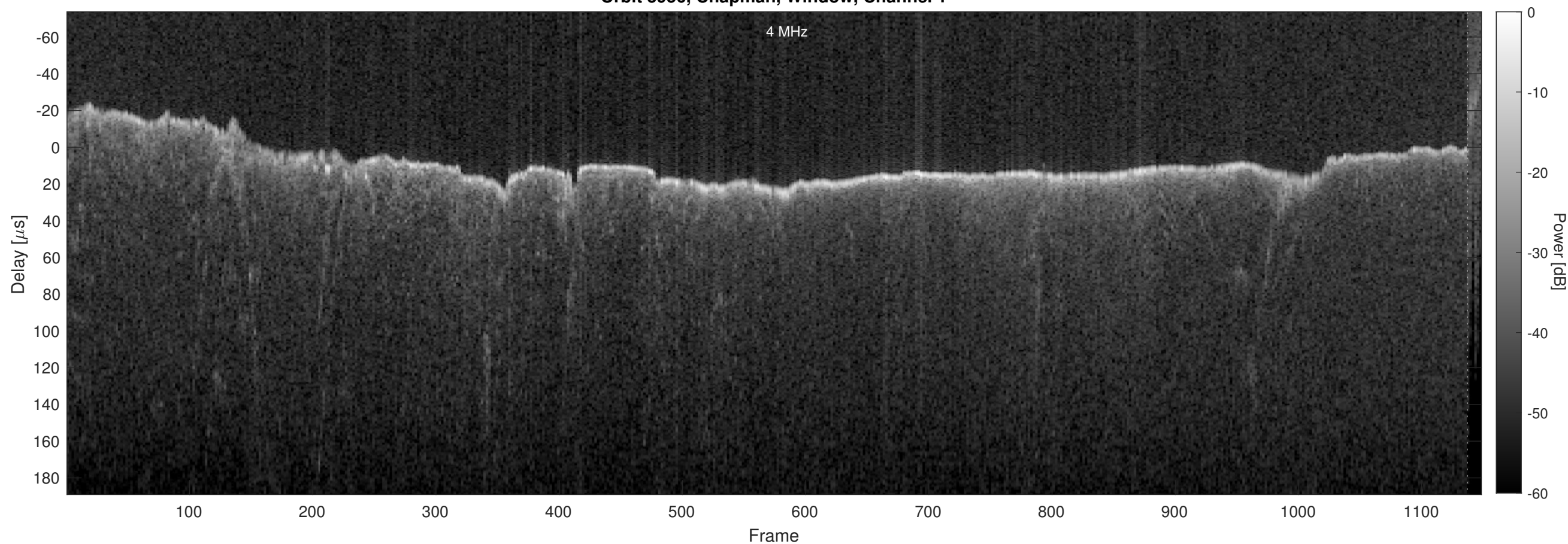
Orbit 3956, Chapman, Window, Channel 2
