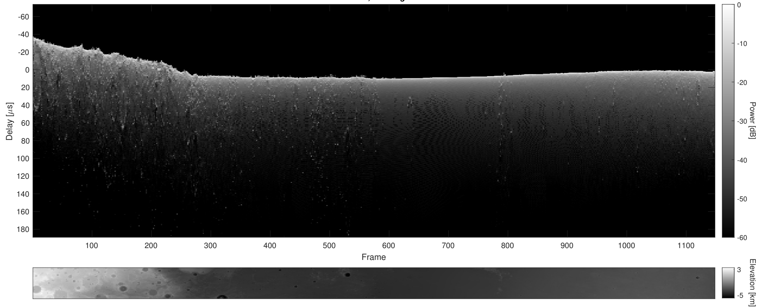
Orbit 3956, Cluttergram
