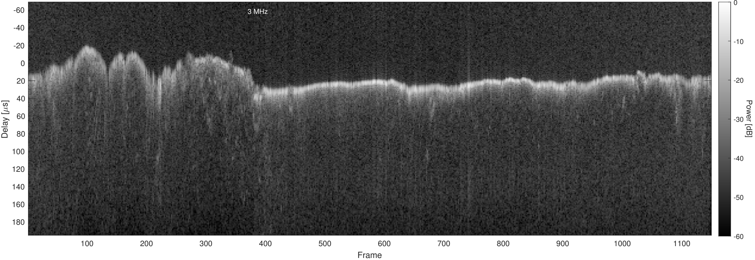
Orbit 3957, Chapman, Window, Channel 2
