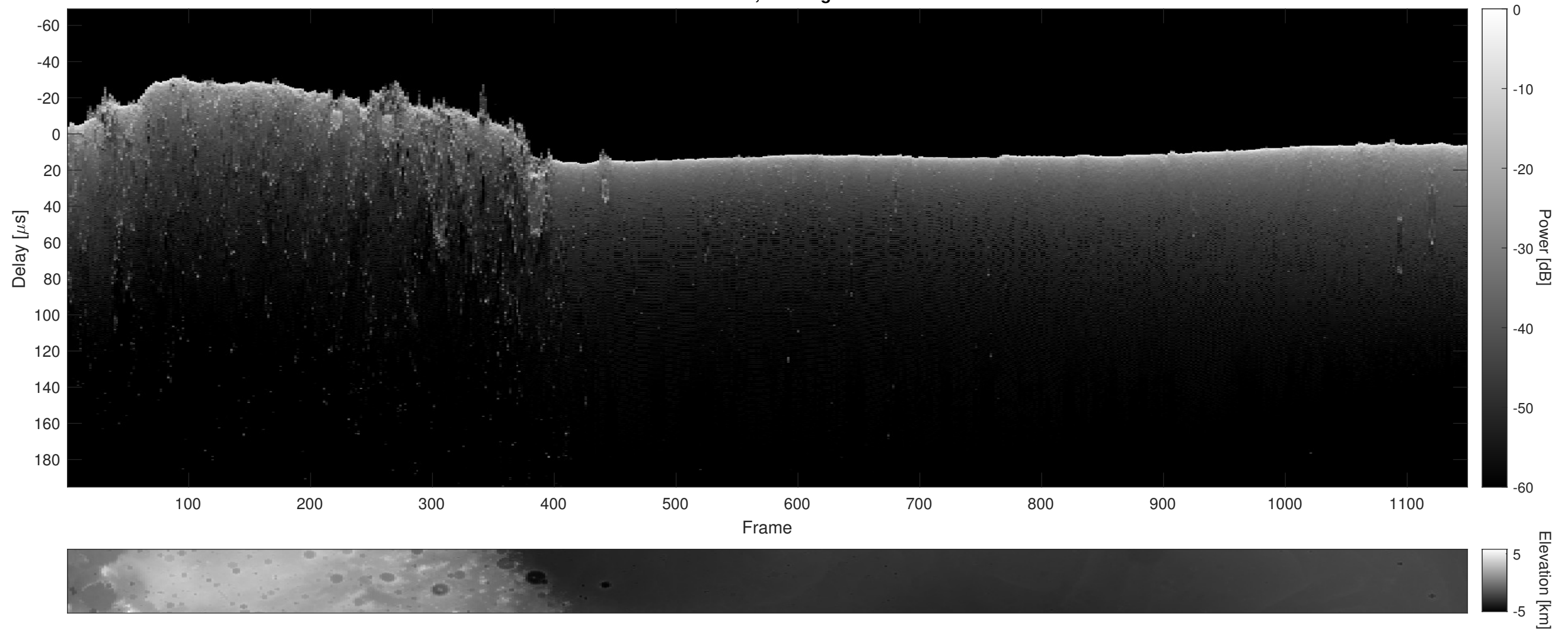
Orbit 3957, Cluttergram
