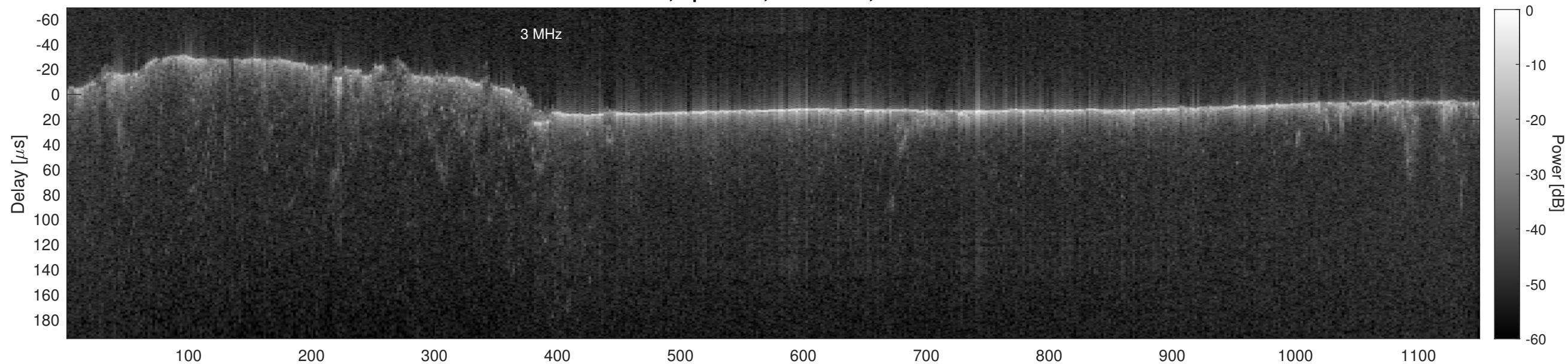
Orbit 3957, Cluttergram
