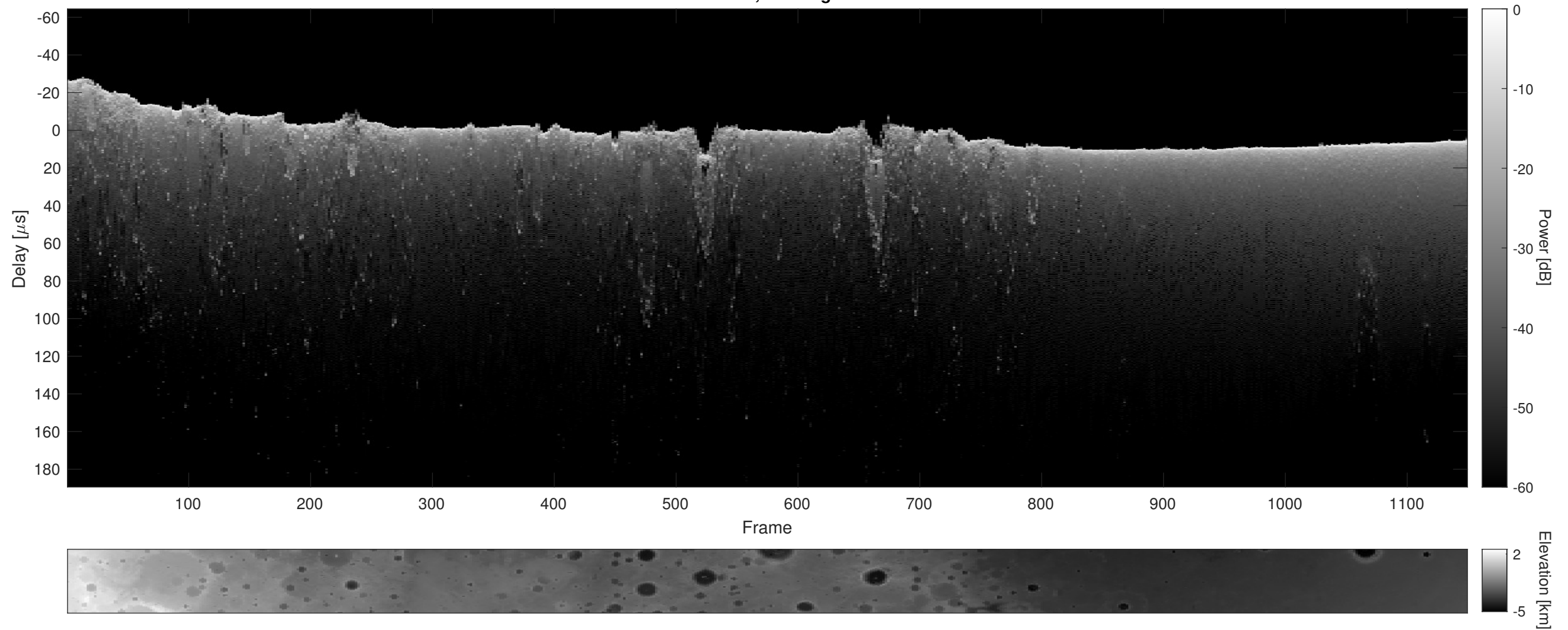
Orbit 3958, Cluttergram
