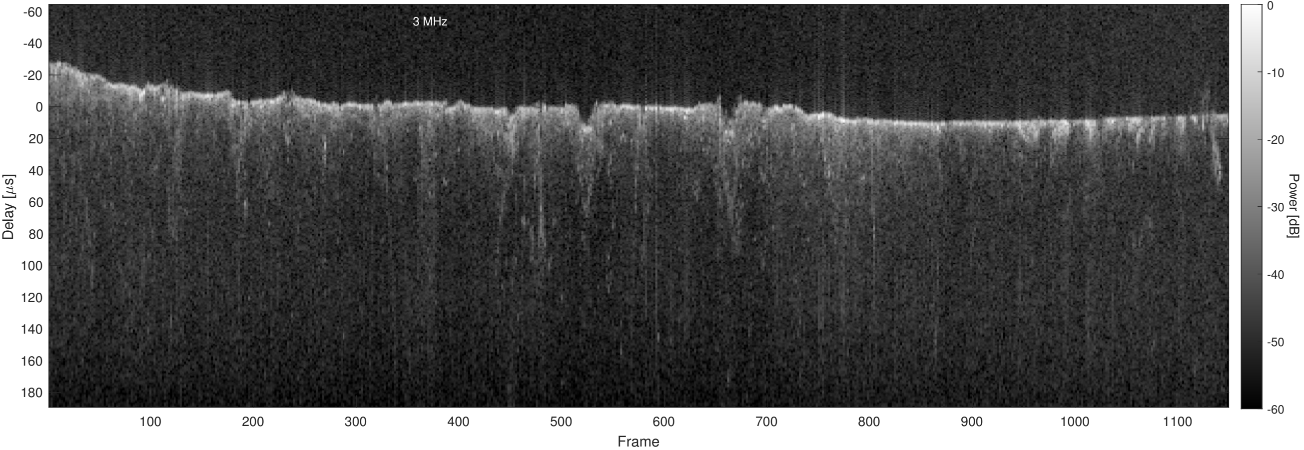
Orbit 3958, Optimized, Window, Channel 2
