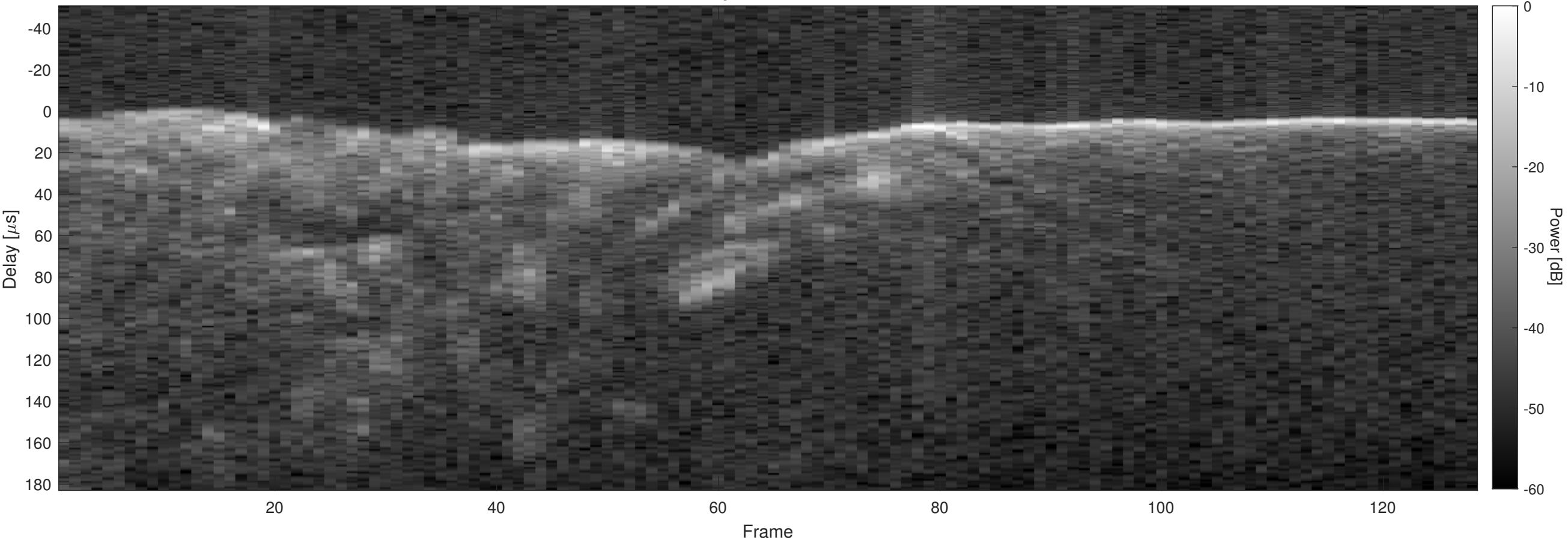
Orbit 3959, Chapman, Window, Channel 2
