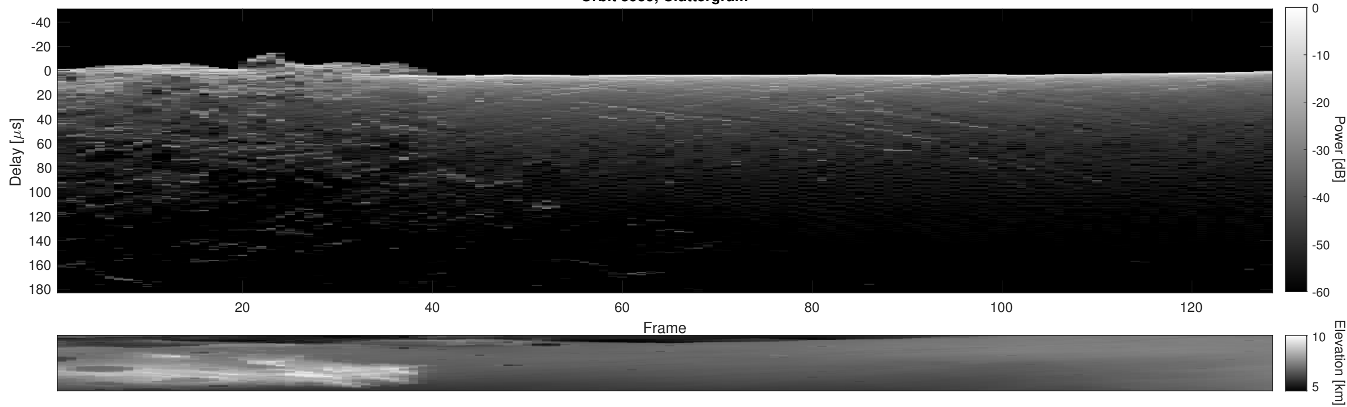
Orbit 3959, Cluttergram
