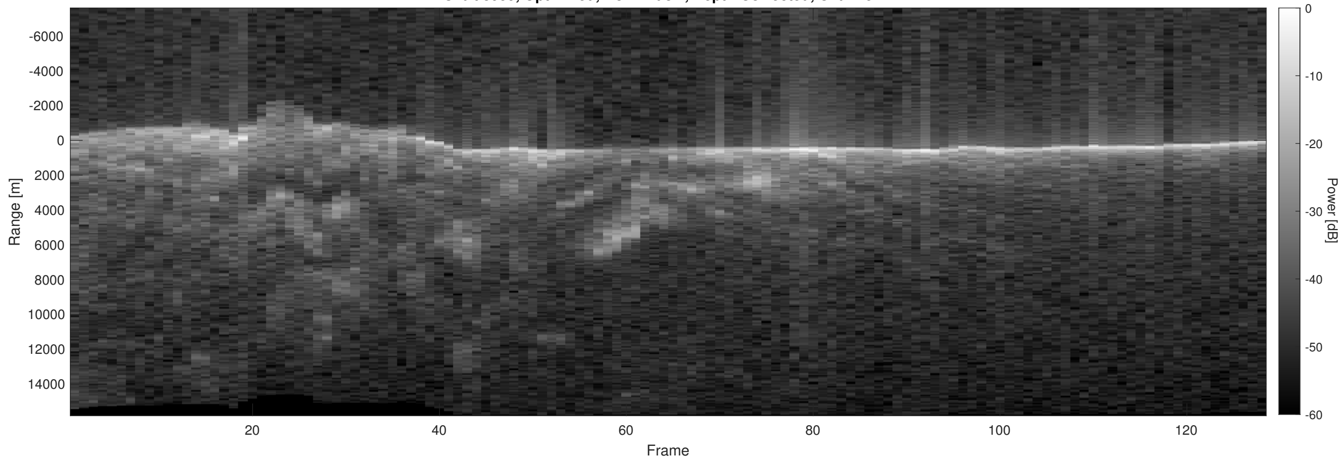
Orbit 3959, Optimized, No Window, Depth-Corrected, Channel 2
