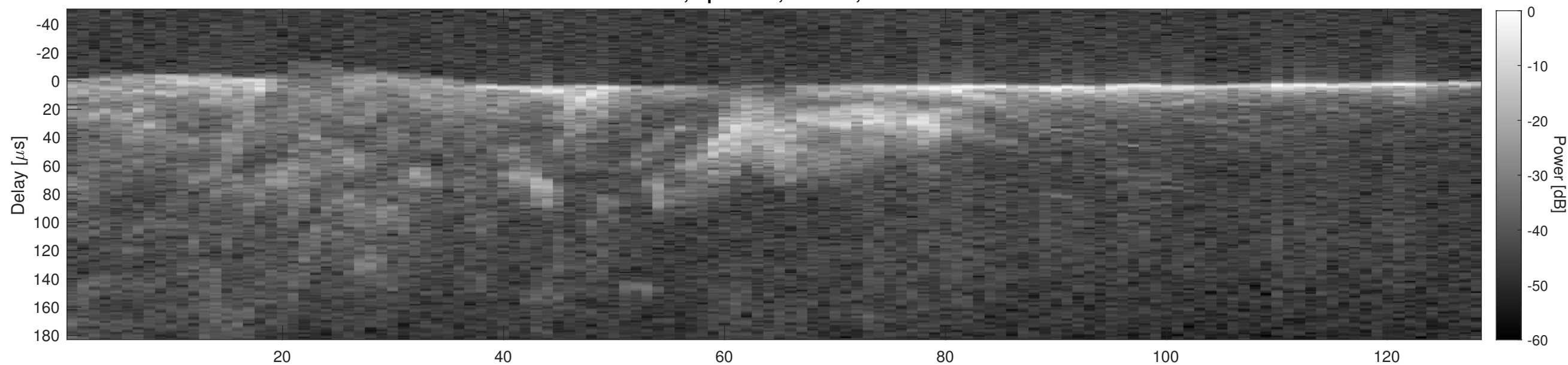
Orbit 3959, Cluttergram
