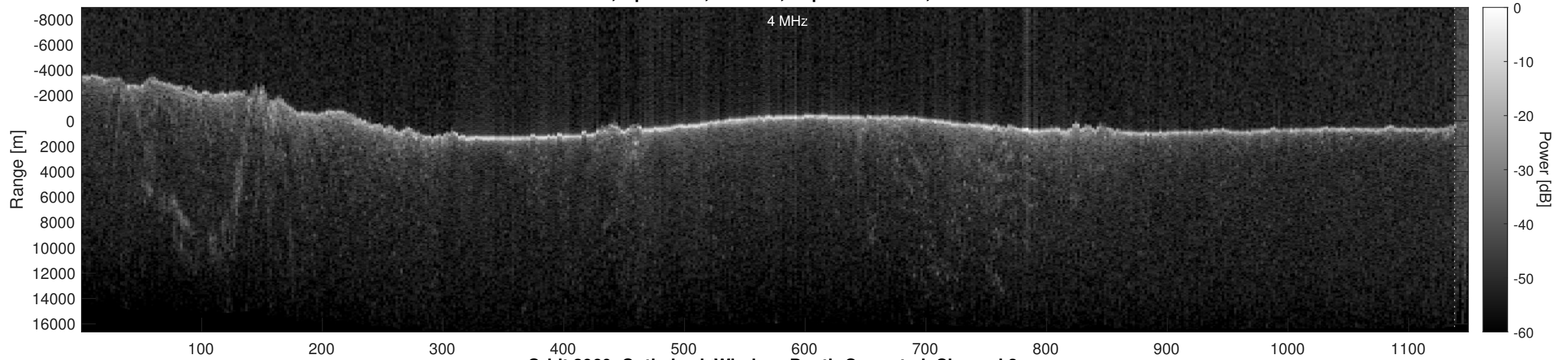
Orbit 3960, Optimized, Window, Depth-Corrected, Channel 2
