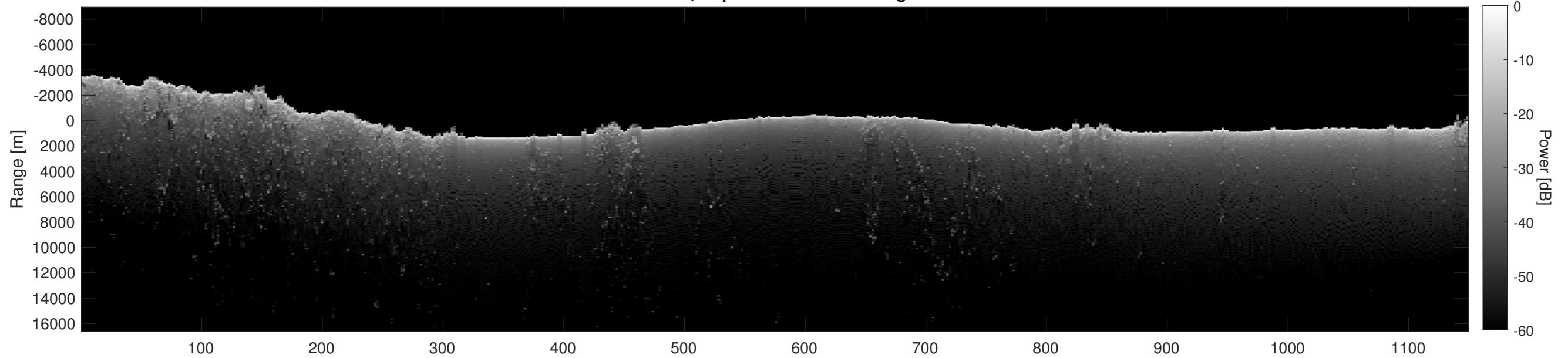
Orbit 3960, Depth-Corrected Cluttergram
