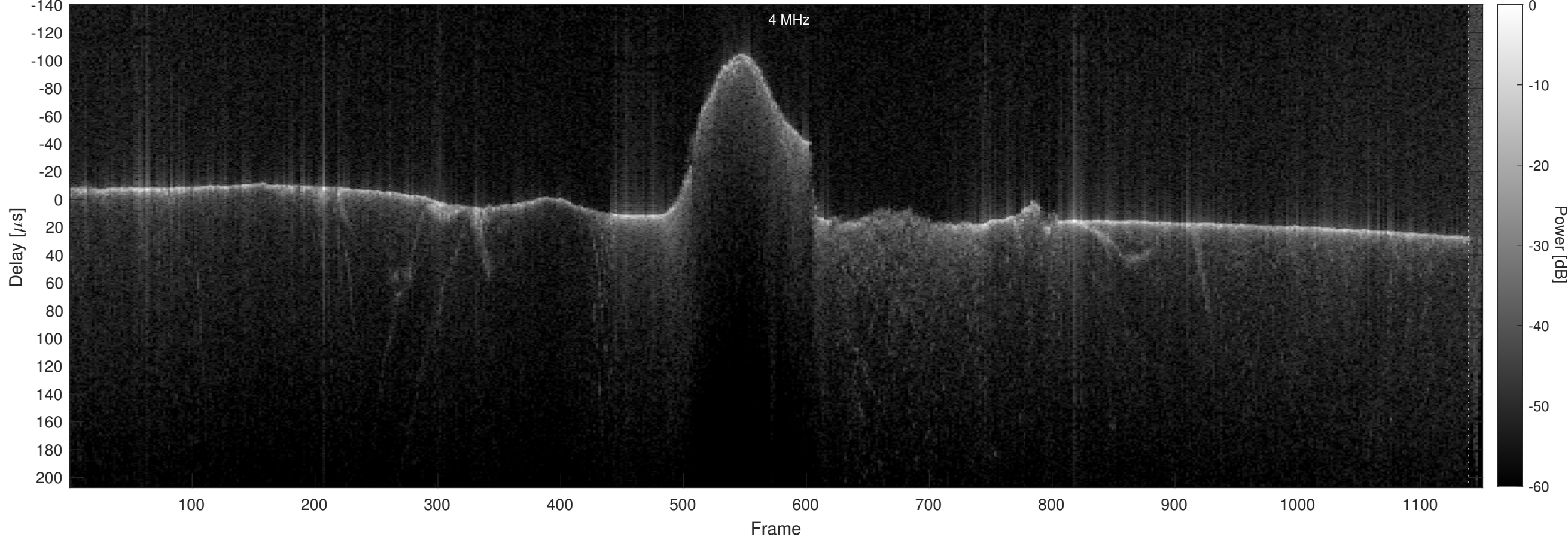
Orbit 3963, Optimized, No Window, Channel 2
