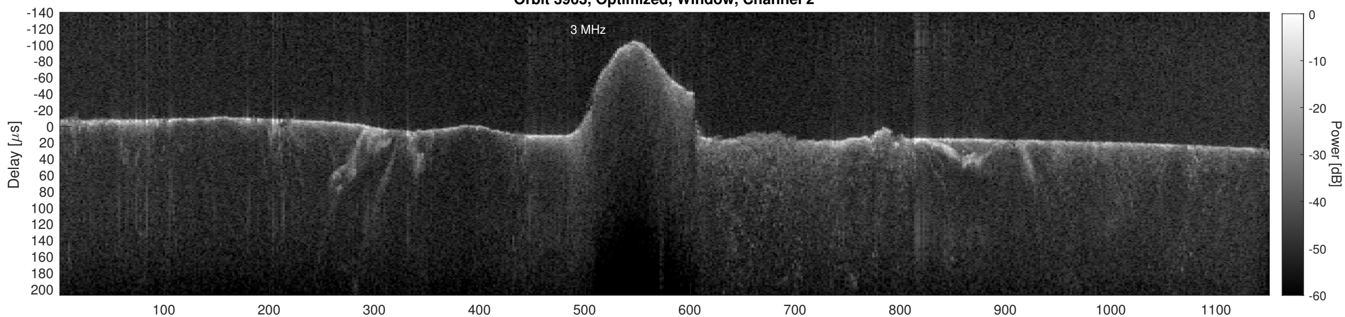
Orbit 3963, Cluttergram
