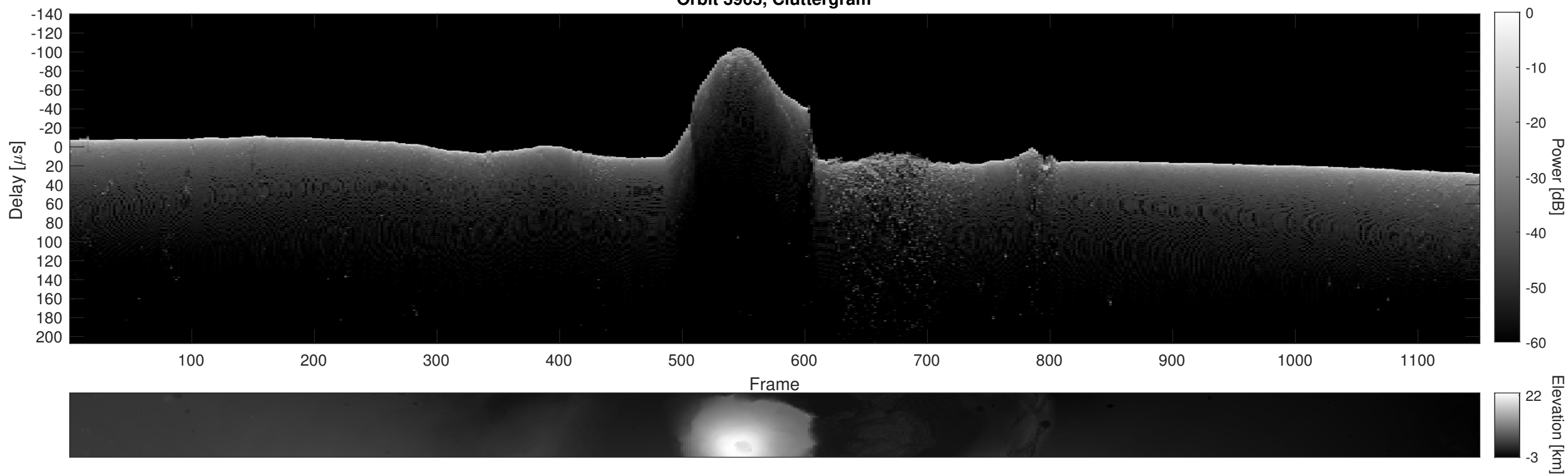
Orbit 3963, Cluttergram
