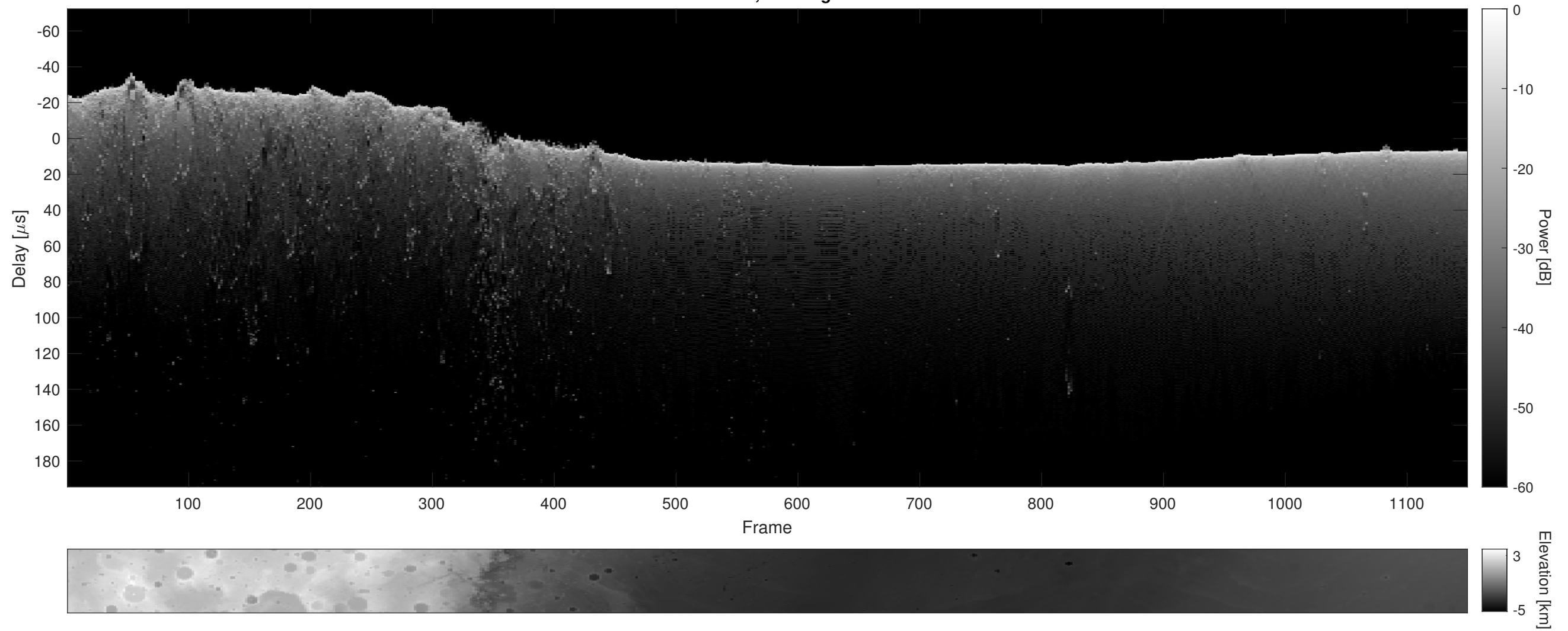
Orbit 3964, Cluttergram
