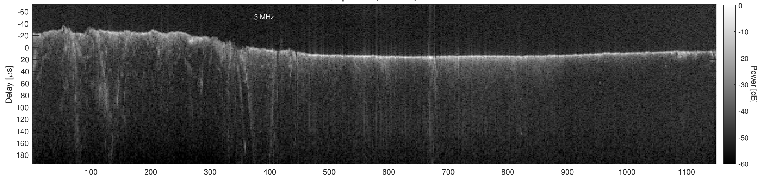
Orbit 3964, Cluttergram
