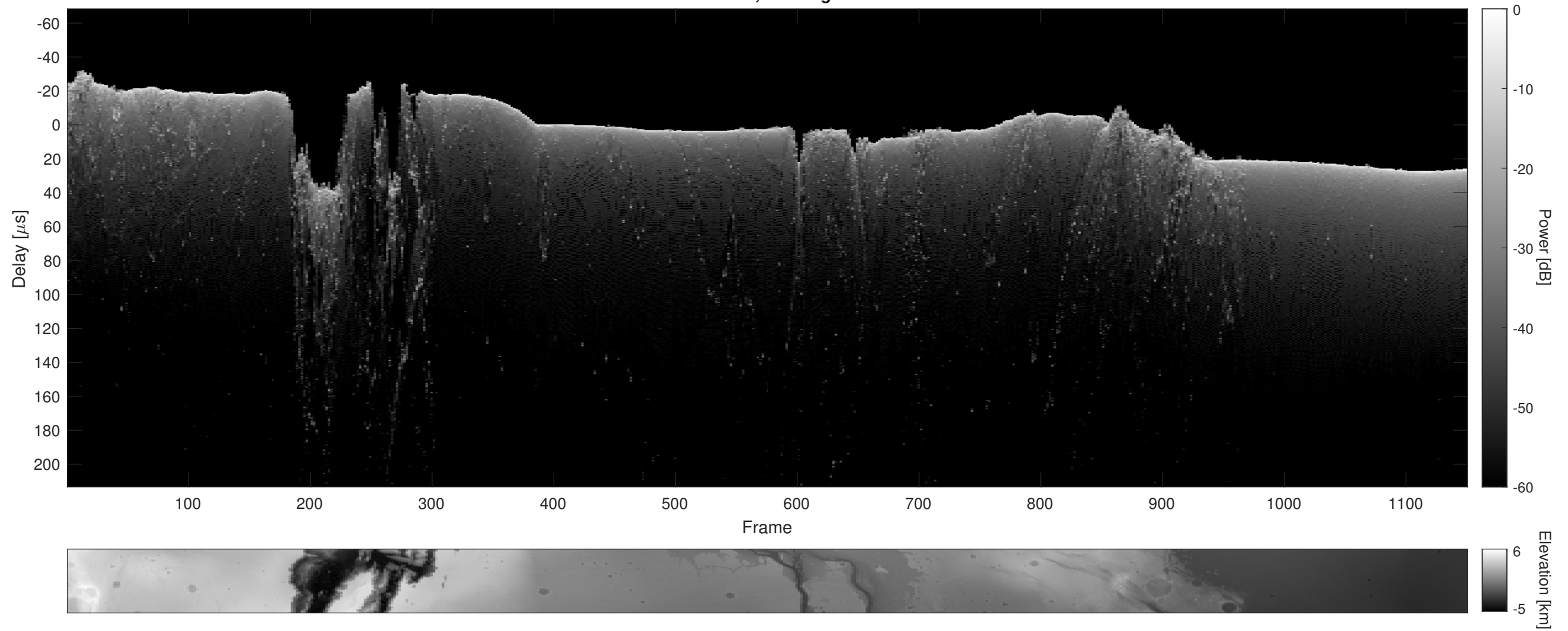
Orbit 3966, Cluttergram
