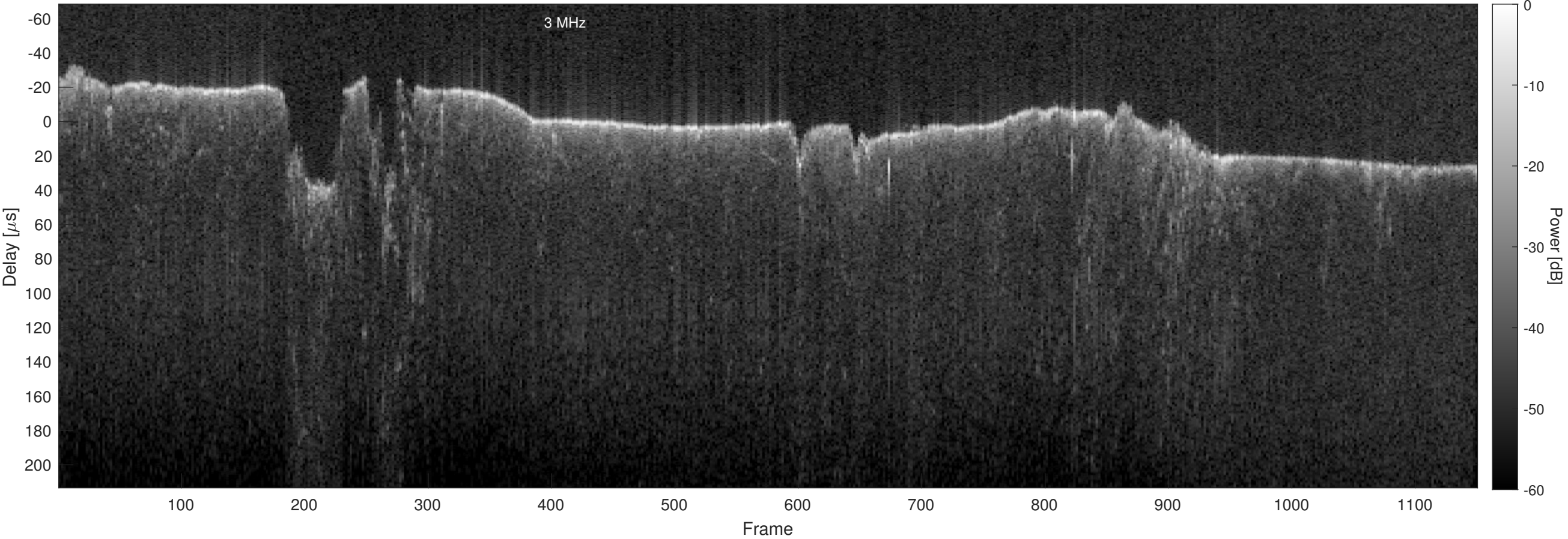
Orbit 3966, Optimized, Window, Channel 2
