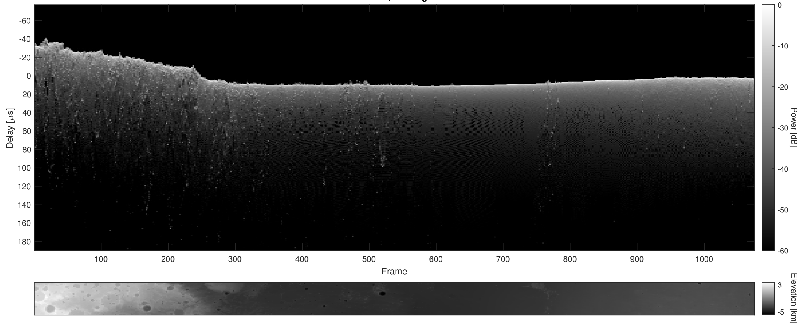
Orbit 3967, Cluttergram
