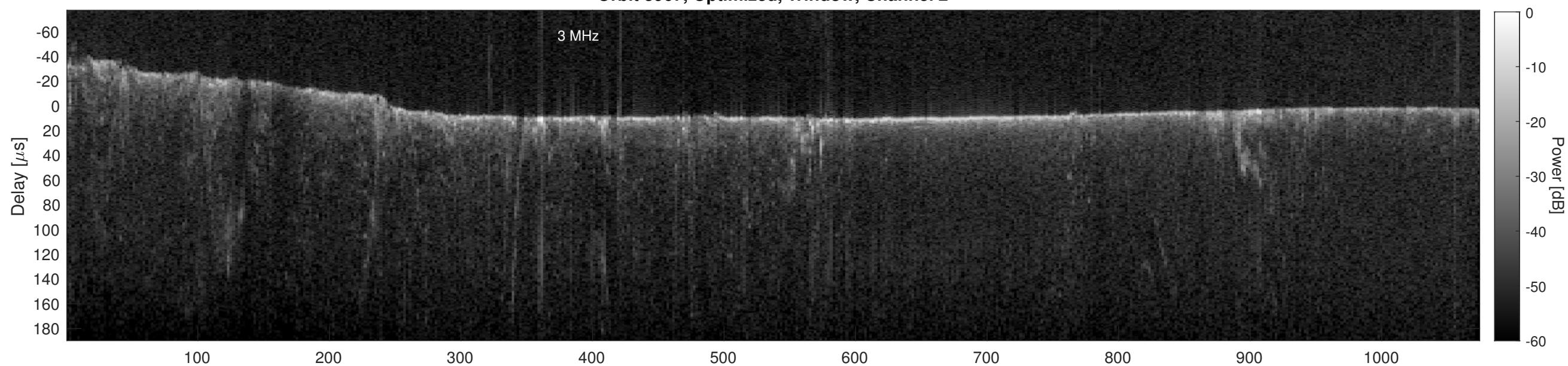
Orbit 3967, Cluttergram
