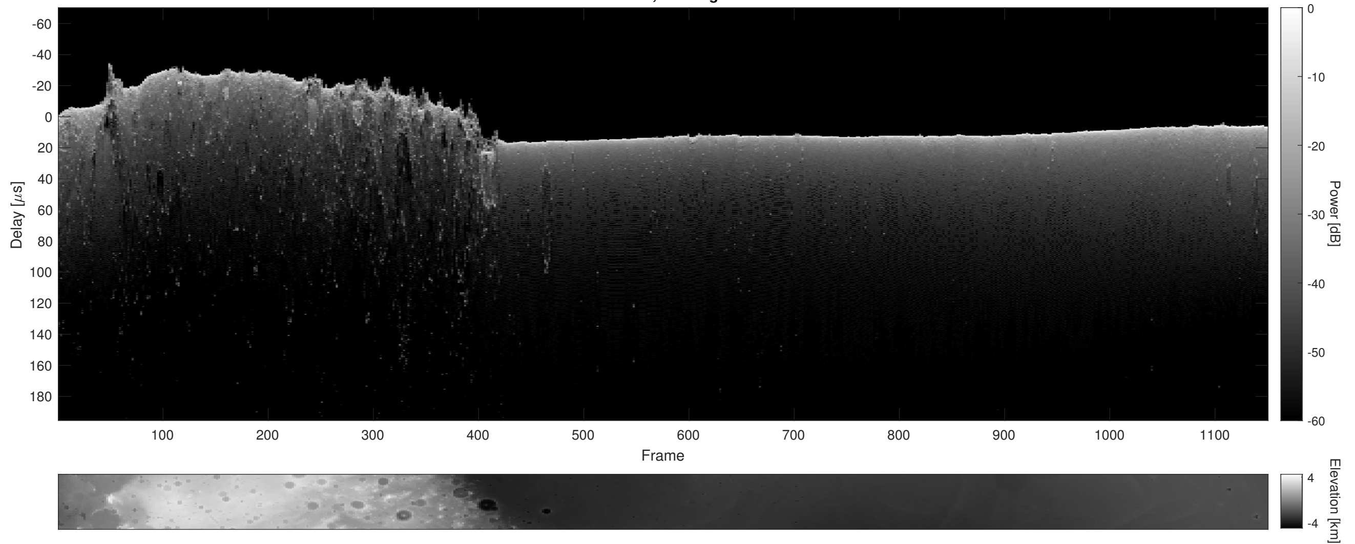
Orbit 3968, Cluttergram
