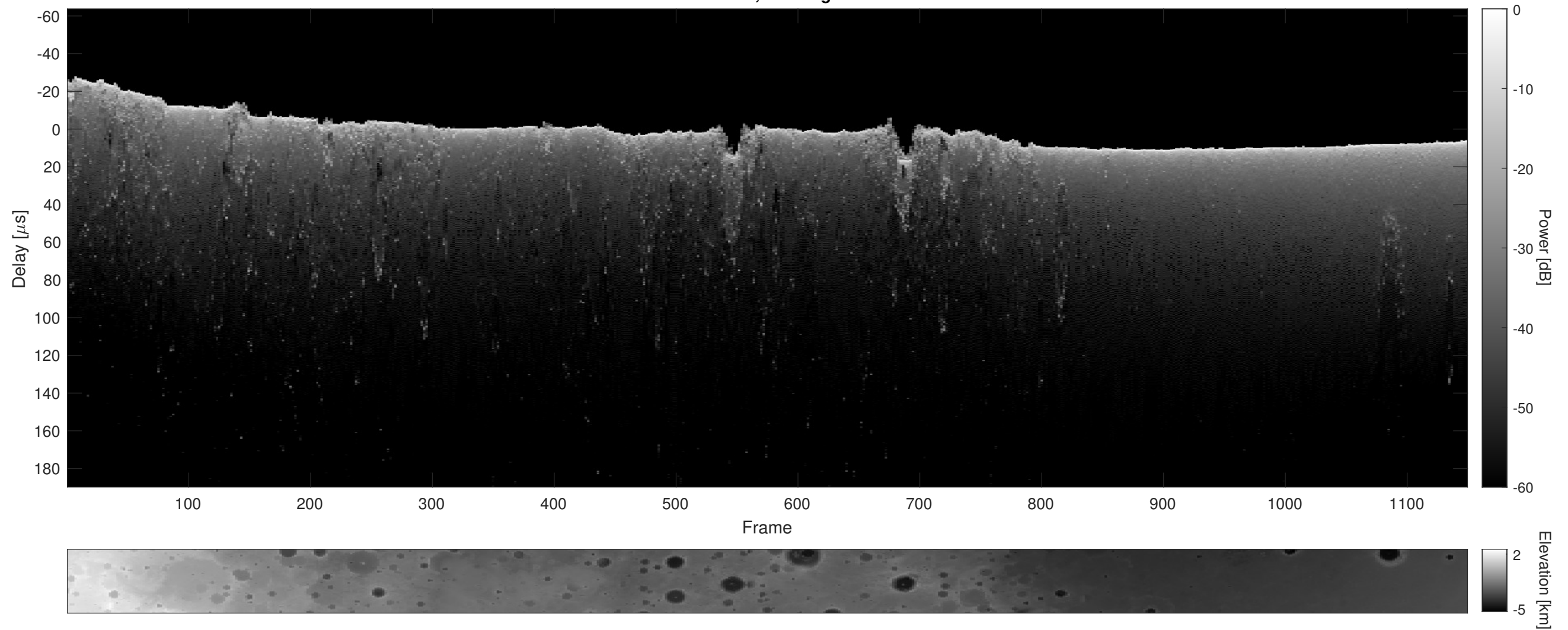
Orbit 3969, Cluttergram
