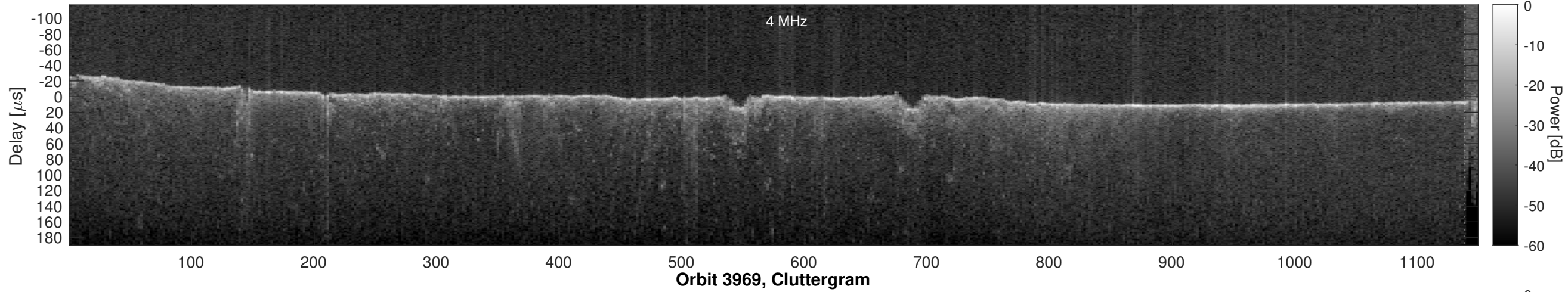
Orbit 3969, Window, Channel 1, Optimized
