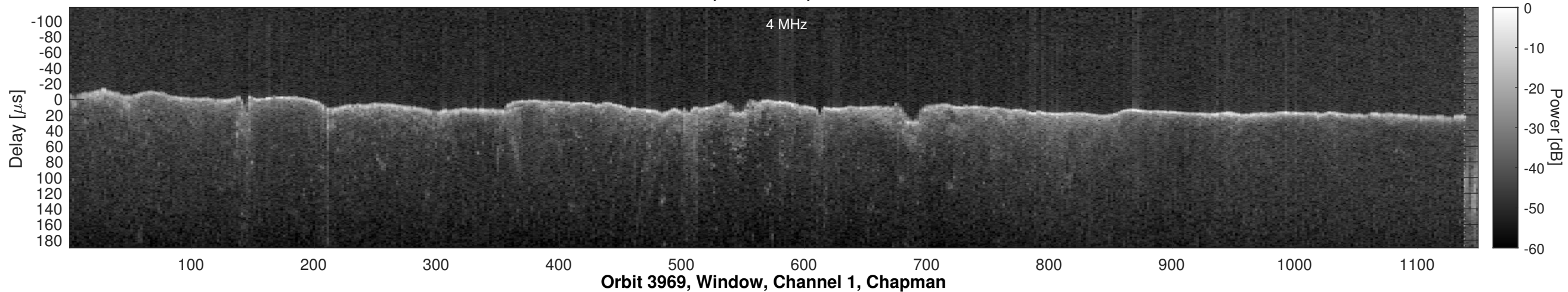
Orbit 3969, Channel 1, Uncorrected
