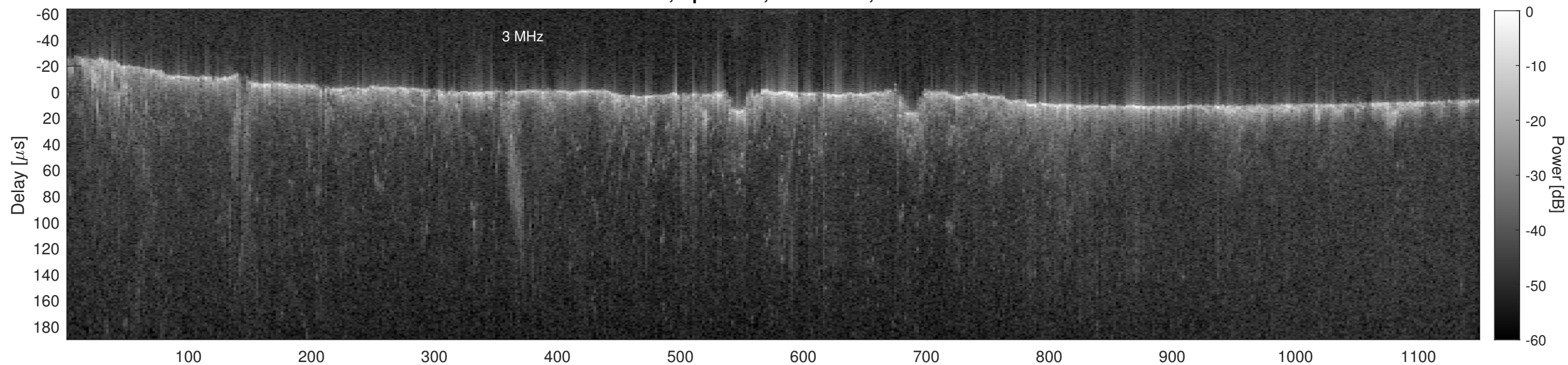
Orbit 3969, Cluttergram
