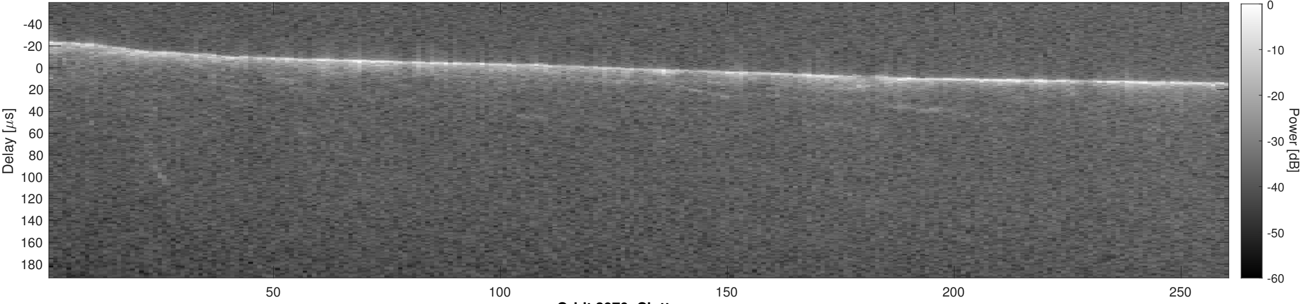
Orbit 3970, Cluttergram
