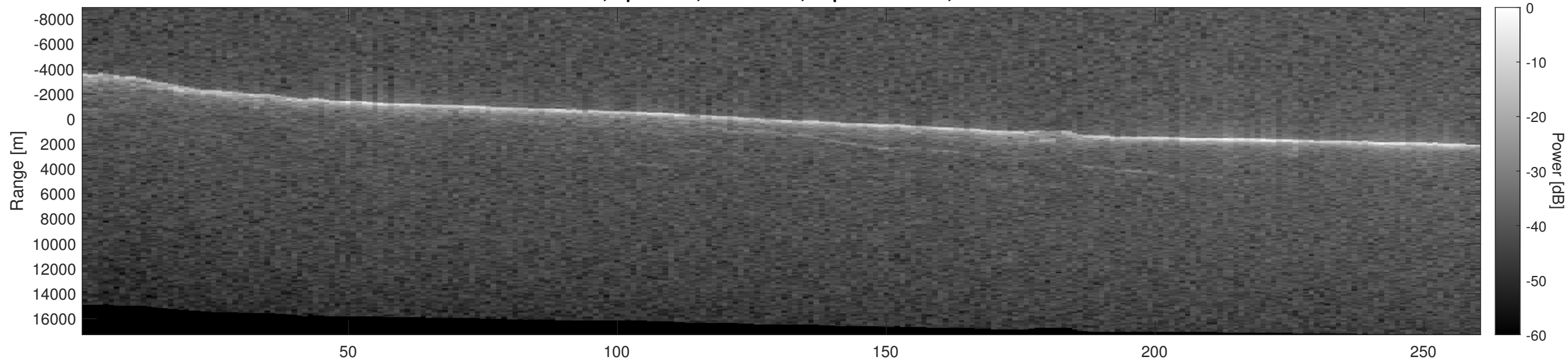
Orbit 3970, Optimized, No Window, Depth-Corrected, Channel 2
