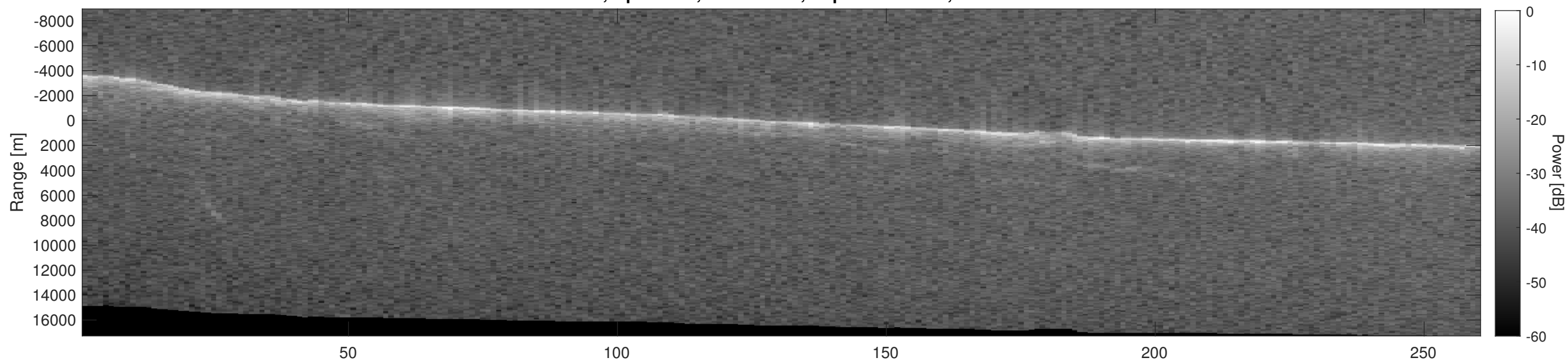
Orbit 3970, Depth-Corrected Cluttergram
