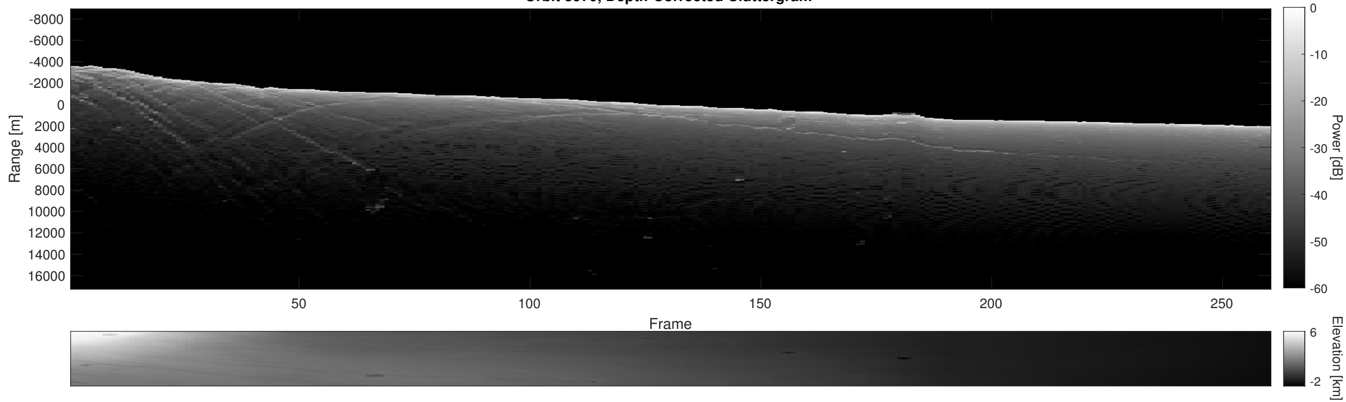
Orbit 3970, Depth-Corrected Cluttergram
